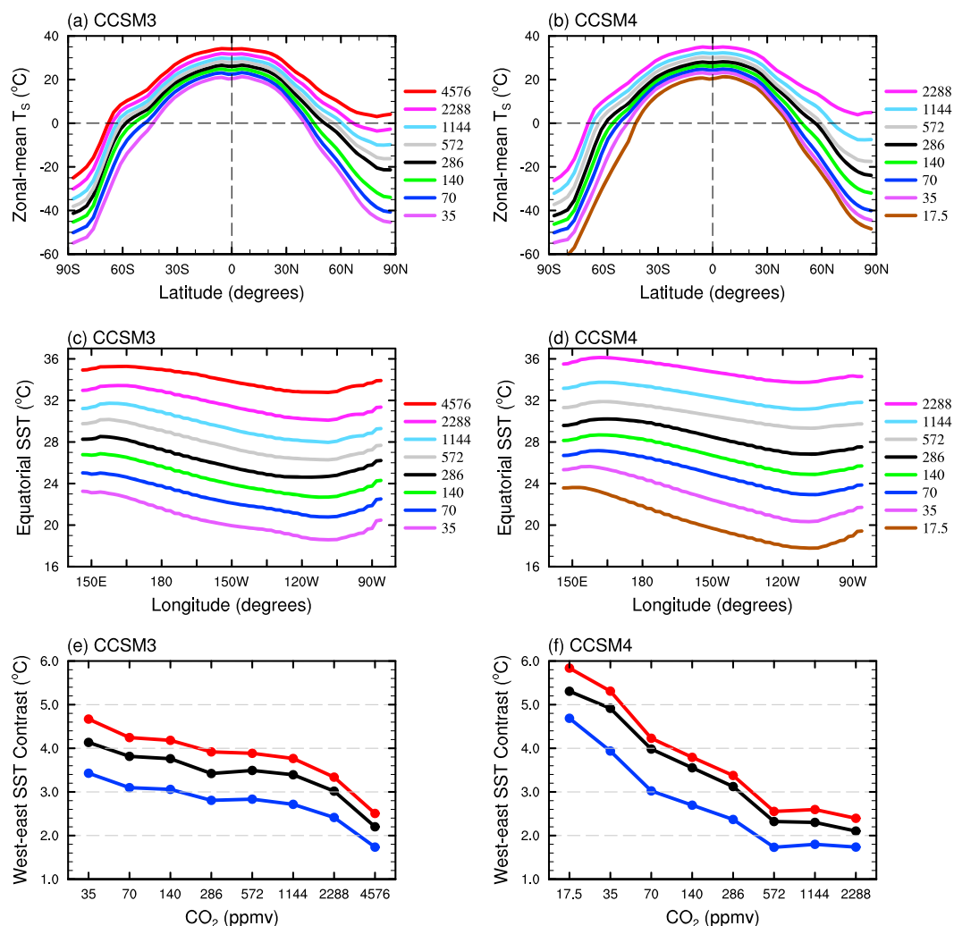
Figure 1. (a, b) Annual- and zonal-mean surface air temperature ( T_s ); (c, d) annual-mean sea surface temperature (SST) along the equatorial Pacific ( 5^{\circ}S-5^{\circ}N ); (e, f) west-east SST contrast. The west-east SST contrast is defined by the maximum minus the minimum (red dots), the difference between [ 5^{\circ}S to 5^{\circ}N , 150^{\circ}E to 170^{\circ}E ] and [ 5^{\circ}S to 5^{\circ}N , 115^{\circ}W to 95^{\circ}W ] (black dots), or the difference between [ 10^{\circ}S to 10^{\circ}N , 150^{\circ}E to 170^{\circ}E ] and [ 10^{\circ}S to 10^{\circ}N , 115^{\circ}W to 95^{\circ}W ] (blue dots). Left column is for CCSM3 and right column for CCSM4. The CO_2 concentrations in CCSM3 are from 35 to 4576 ppmv and in CCSM4 from 17.5 to 2288 ppmv.
