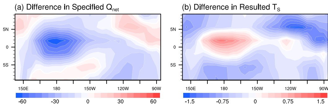
Figure 5. (a) Difference in the specified surface heat flux into the ocean ( Q_{net} , W m^{-2} ) and (b) difference in the resulted surface temperature ( T_s , K), simulated by the atmospheric component of CCSM3, which is CAM3, coupled to a 50 m slab ocean. The CO_2 concentration is 4576 ppmv in both experiments.
