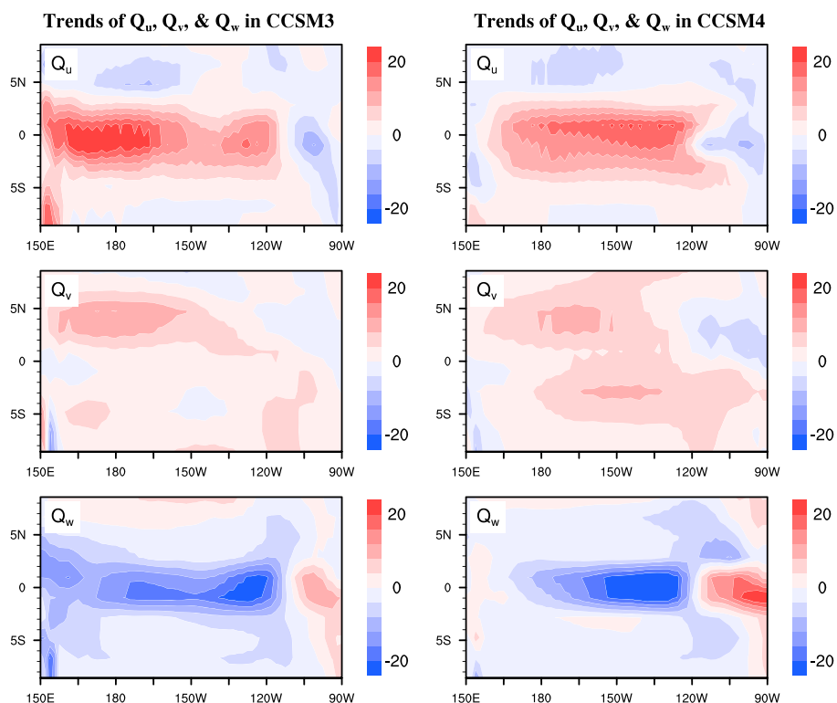
Figure 11. Trends of the divergences of (top row) zonal ocean heat transport ( Q_u ), (middle row) meridional ocean heat transport ( Q_v ), and (bottom row) vertical ocean heat transport ( Q_w ) vertically integrated from the sea surface to the depth of 75 m, in response to doubling atmospheric CO_2 concentration in CCSM3 (left column) and CCSM4 (right column). Positive values imply heating of the ocean surface layer. The contour interval is 2 W m^{-2} . The calculation follows the method of Dinezio et al. [2009].
