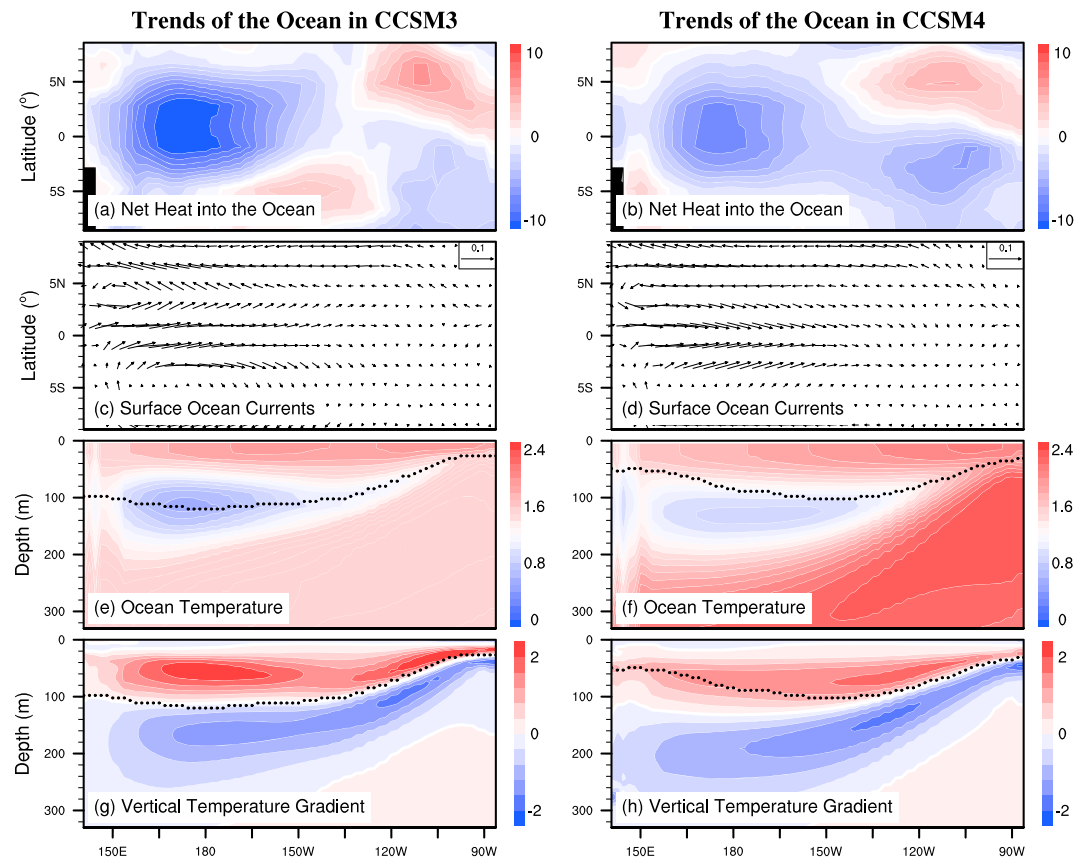
Figure 10. Linear trends of the tropical Pacific Ocean for each doubling of CO 2 concentration. (a, b) Net heat flux into the ocean, (c, d) surface ocean currents, (e, f) upper ocean temperature, and (g, h) vertical ocean temperature gradient. The units are, respectively, W m -2 , 0.1 m s -1 , K, and 0.01 K m -1 for each doubling of CO 2 concentration. The black dots in Figures 10e–10h are the thermocline of the control experiments for the preindustrial condition. Note that Figures 10a and 10b are the same as Figures 4m and 4n, but the resolution is for the ocean grid, which is higher than that for the atmosphere grid.
