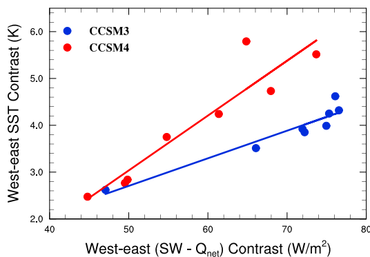
Figure 6. Relationship between west-east ( SW - Q_{net} ) contrast and west-east SST contrast. SW is all-sky surface net shortwave flux, and Q_{net} is net heat flux into the ocean (equation (1)). Blue dots are for CCSM3 and red dots for CCSM4. The lines are corresponding line regressions. The west-east contrast is defined by the difference between [5^\circ S to 5^\circ N , 150^\circ E to 170^\circ E] and [5^\circ S to 5^\circ N , 115^\circ W to 95^\circ W] .
